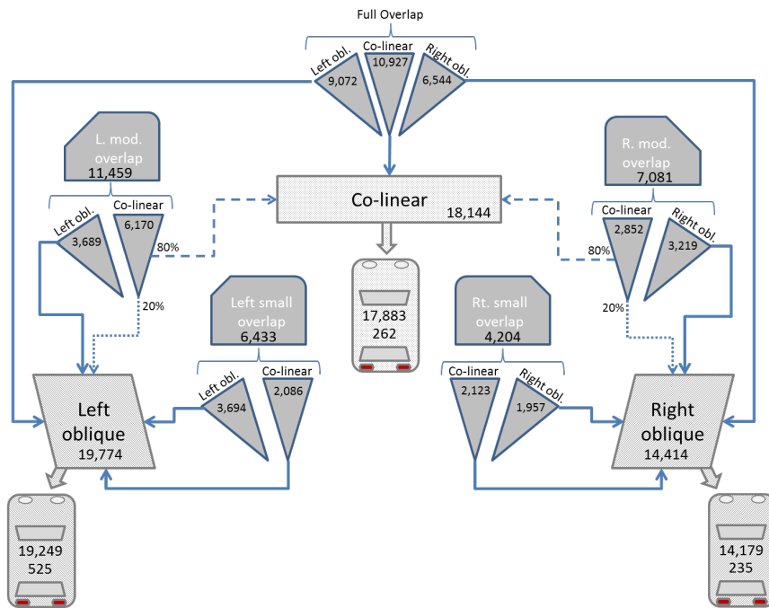
Figure I-2: Breakdown of MAIS 2+ or fatal frontal crash occupants by overlap and obliquity. Counts represent weighted annualized totals from 2000-2013 NASS-CDS for front and second row occupants. Counts displayed are front row and second row combined, except in the vehicle diagrams that include the counts broken out by seat row.
