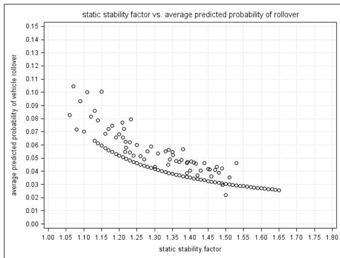
Figure 4. Current and new rollover risk curve
