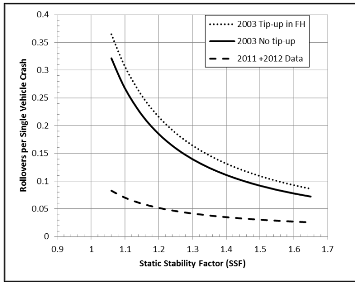
Figure 4. Current and new rollover risk curve
