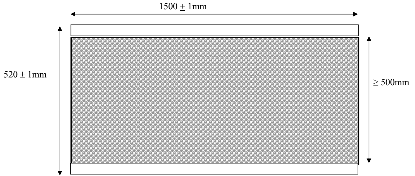
Figure 5 - Front View
