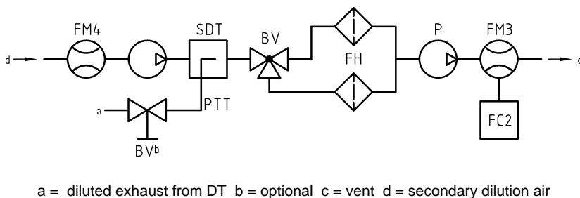
a = diluted exhaust from DT b = optional c = vent d = secondary dilution air
