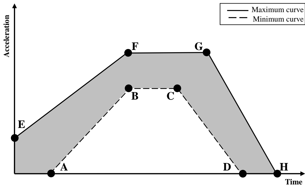
Figure 14 Generic description of test pulses
