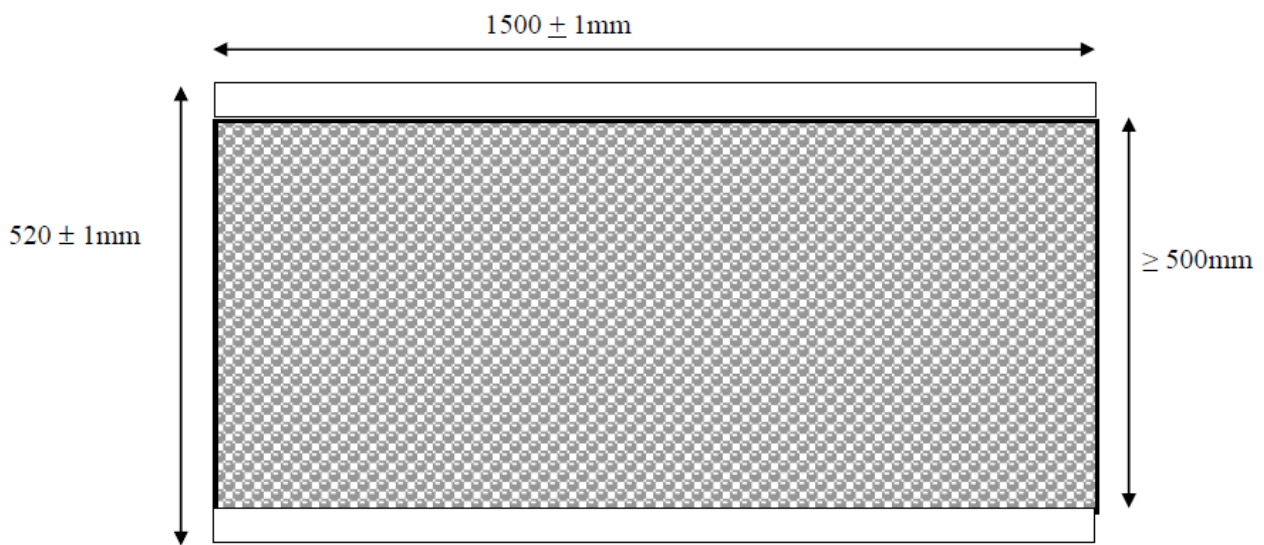
Figure 5 - Front View
